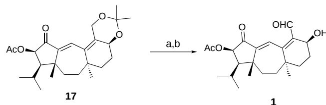
Scheme 6. Synthesis of 1 . a) PPTS, MeOH, 70 °C; b) PhI(OAc) 2 , TEMPO, CH 2 Cl 2 , 59–65 % overall yield. TEMPO = 2,2,6,6-tetramethyl-1-piperidinyloxy, free radical.
